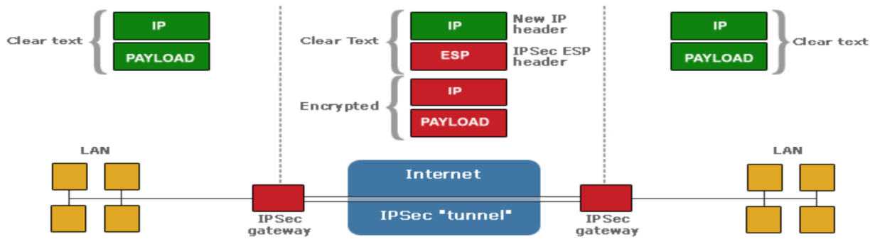
Figure 2: IPsec contains a gateway and a tunnel in order to secure communications.
